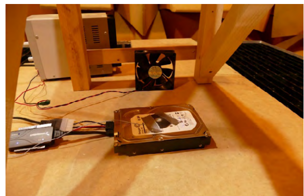
Figure 2: Photograph of the test set-up showing the HDD on an MDF board in the anechoic chamber at Michigan Technological University with the speakers placed 0.5 m above the HDD (left). The surface mount microphone, a fan used for cooling the HDD and the USB 3.0 cables used for performance test (right).
